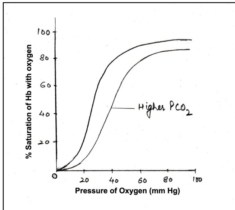
Fig.2. 5 Oxygen-hemoglobin dissociation curve: Increase in concentration/ pressure of \text{CO}_2 shifts the curve to the right
