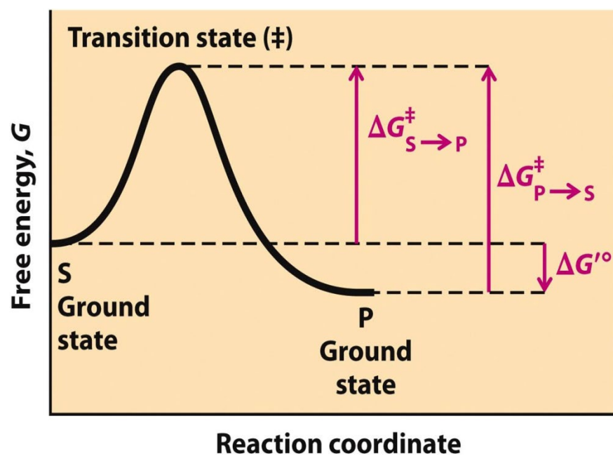
Figure No. 13.1 (A) Reaction coordinate diagram for a chemical reaction. (B) Reaction coordinate diagram comparing enzyme- catalyzed and uncatalyzed reactions
