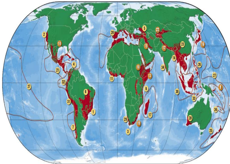
Fig.6.3 Hot –spot area
