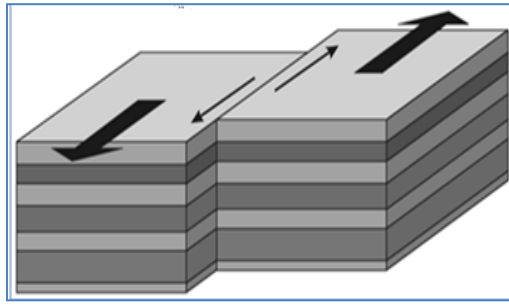
Fig.9.3- Showing Strike slip fault
