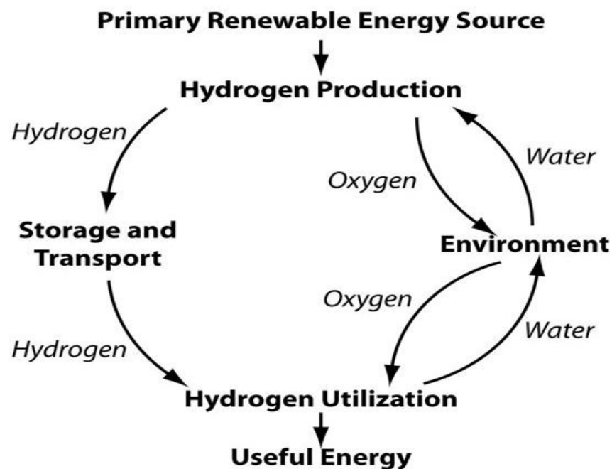
Figure 5.3. Hydrogen Cycle
