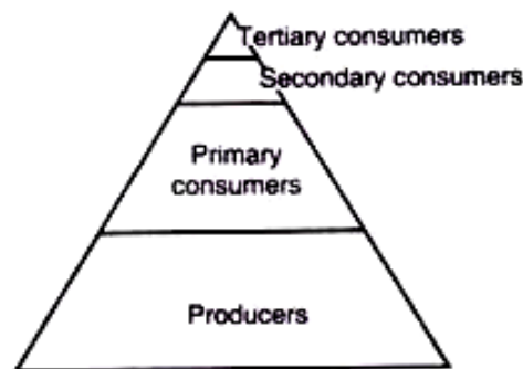
Fig .3.12 Pyramid of energy
