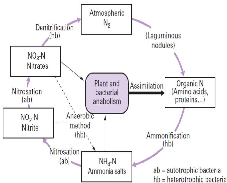
Figure 5.1. Nitrogen Cycle
