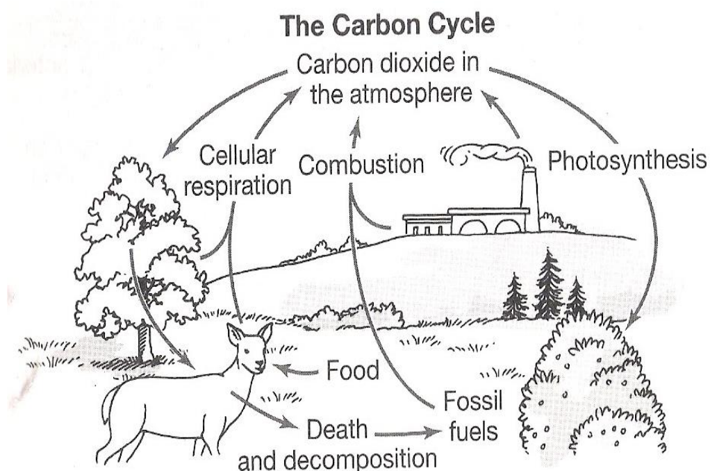
Figure 5.2. Carbon Cycle
