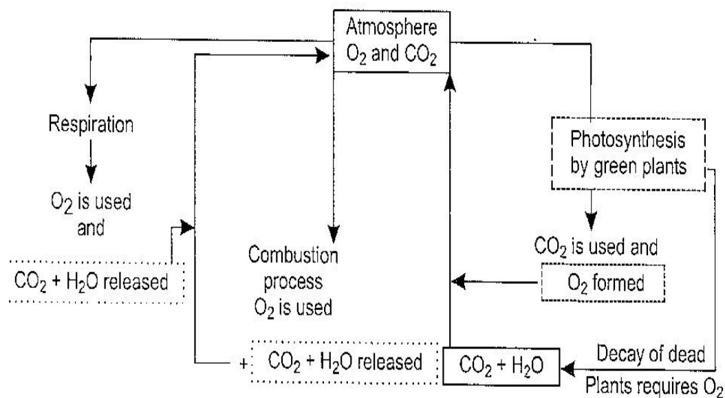
Figure 5.4. Oxygen Cycle
