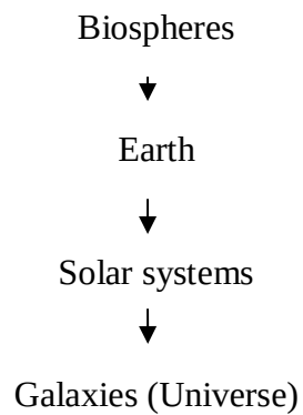
Flow diagram of Levels of organization with in the Earth
