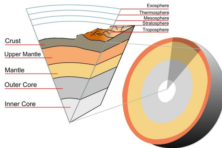
Fig4. 4: Showing different layers in Earth interiors.
