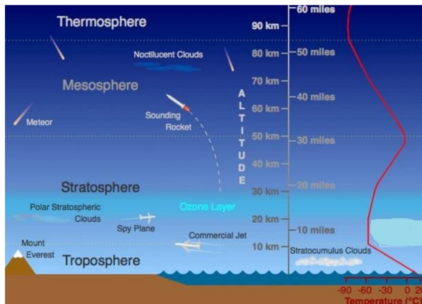
Fig 4.2: Showing the different strata of the Atmosphere
