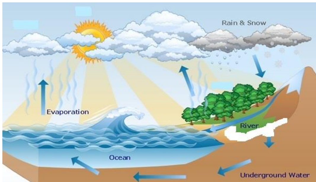
Fig 4.3. Showing the water cycle and Hydrosphere.
