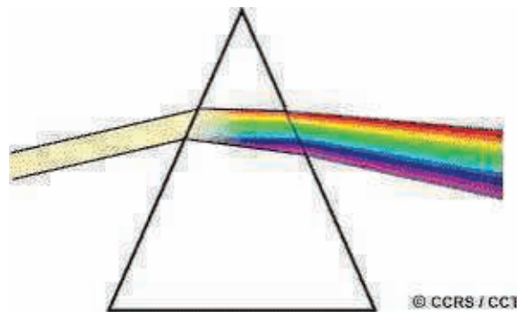
Fig. 1.6: Visible spectrum
