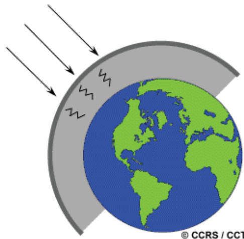
Fig. 1.13: Absorption
