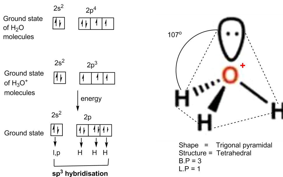
Fig 4.21 Overlapping of filled sp 3 hybrid orbital of O-atom in H 2 O and empty 1s orbital of H + ion to form H 3 O + ion
