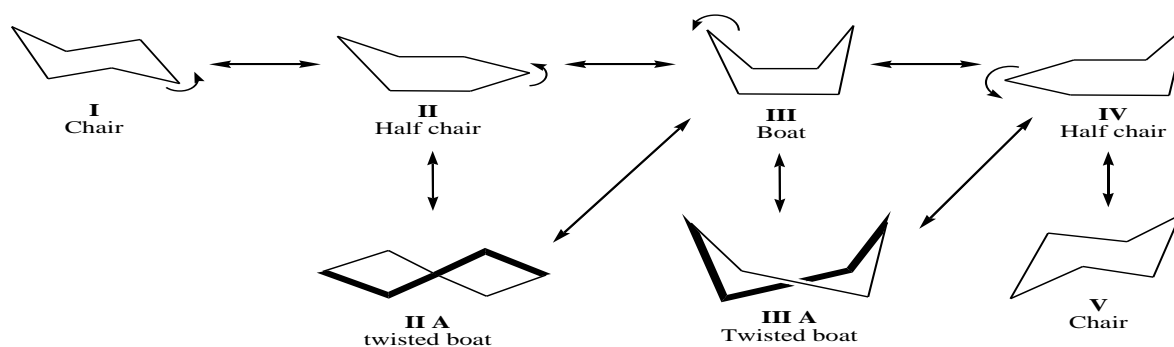
Scheme 1: Conformational analysis of cyclohexane
