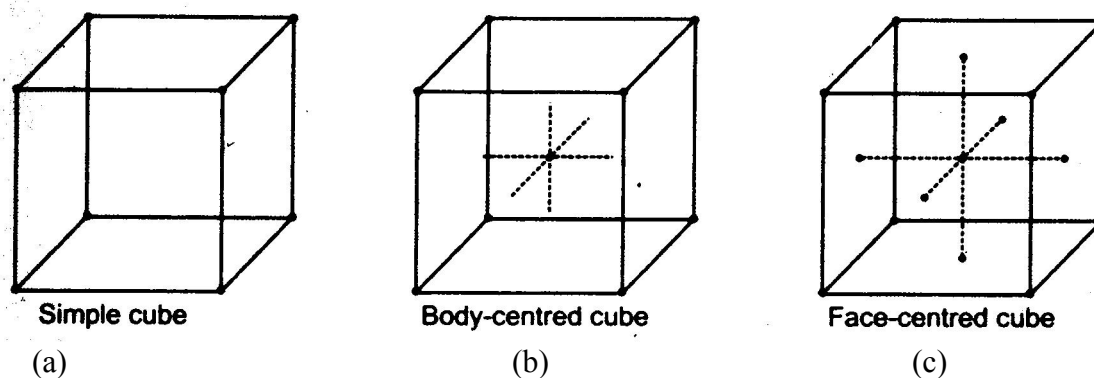
Fig 12.4 Three cubic unit cells
