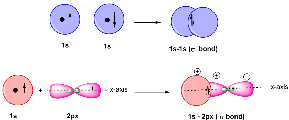
Fig 4.2 overlapping of two s-orbitals along molecular axis
