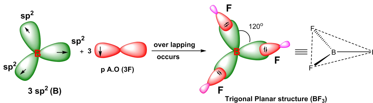
Fig 4.10 formation of three \sigma covalent bonds by the overlapping of sp^2 hybrid orbitals of B-atoms and 2p -orbitals of 3F -atoms
