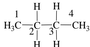
Figure 7.2: Butane molecule
