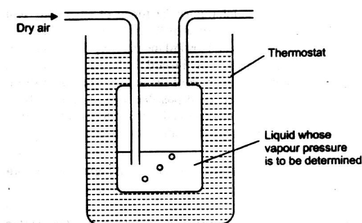
Fig.11.13 Dynamic method
