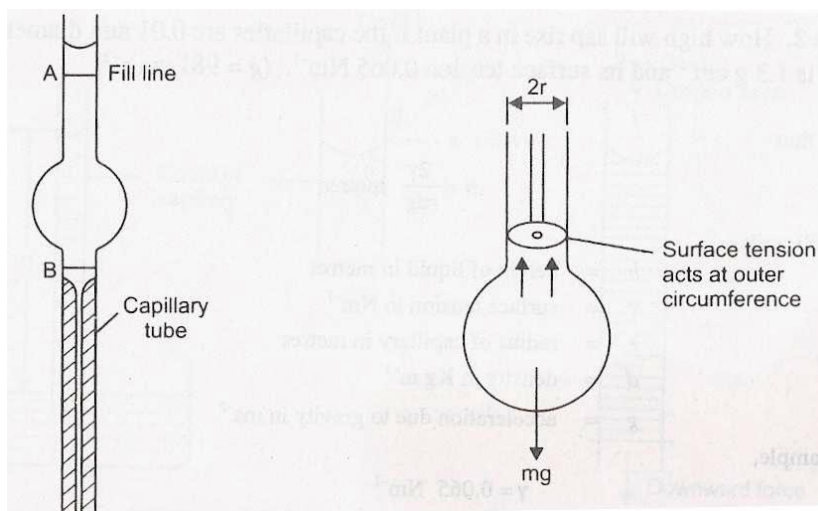
Fig 16.2: Stalagmometer
