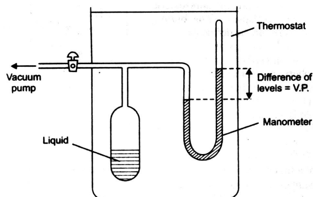
Fig 11.12 Determination of vapour pressure by static method
