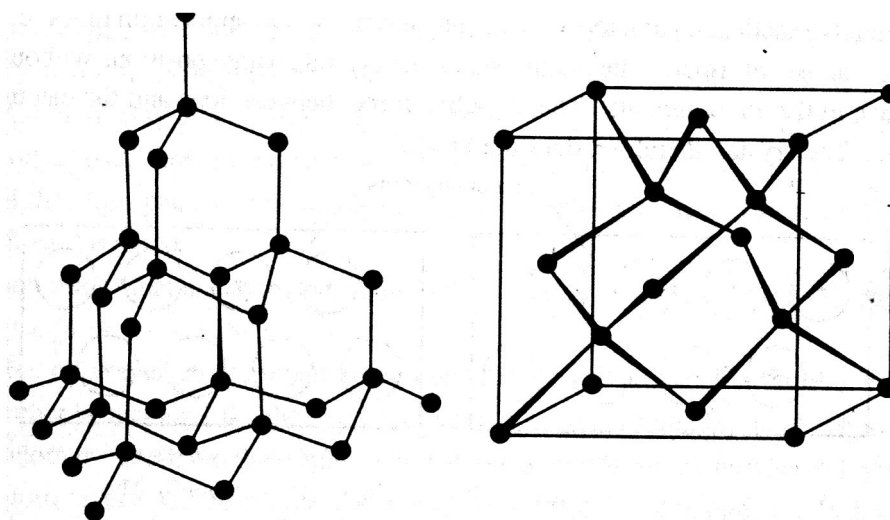
Fig 12.14 crystal structure of diamond
