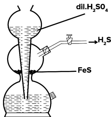
Kipp's apparatus
