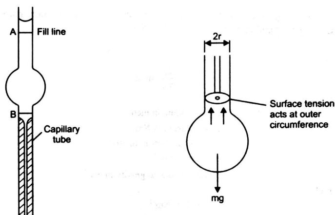
Fig. 11.16 determination of surface tension by drop-pipette
