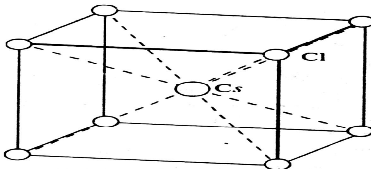
Fig 12.13 Cesium chloride crystal lattice
