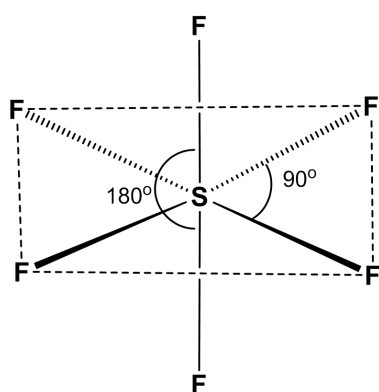
Octahedral complex
