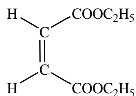
diethyl maleate
