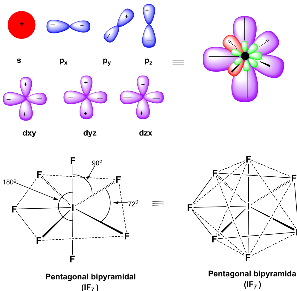
Fig 4.17 Formation of seven sp^3d^3 hybrid orbitals from the mixing of one s , three p and three d -orbitals of the central atom
