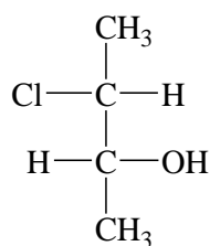
Threo
