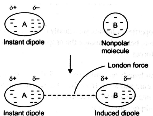
fig 11.8 Explanation of London forces
