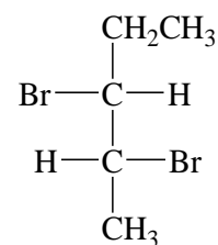
Threo
