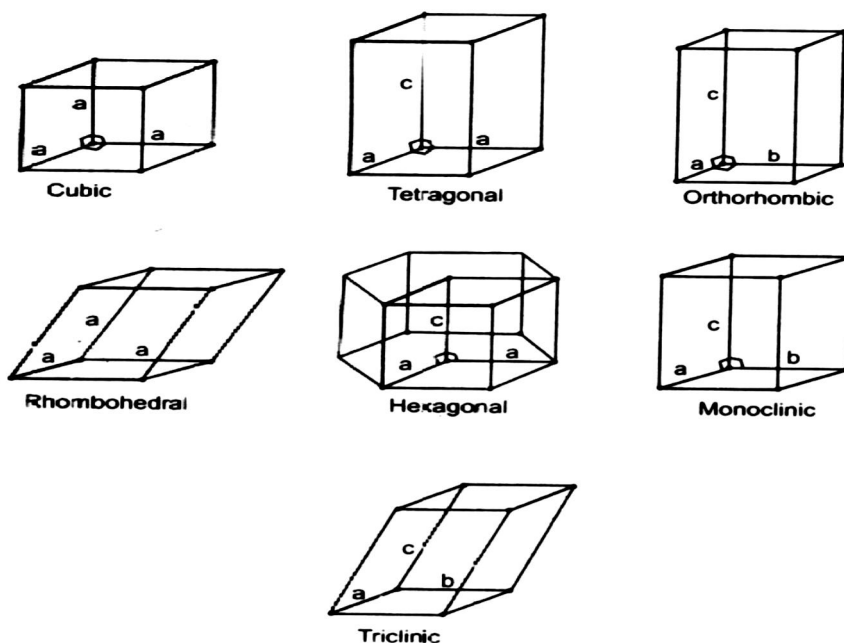
Fig 12.7 seven crystal systems
