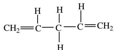
Penta-1,4-diene
