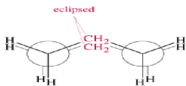
Newman projection
