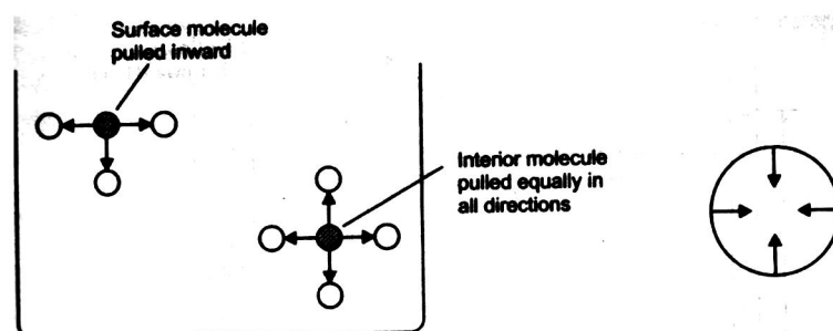
Fig. 11.14 molecular attractions
