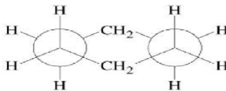
Newman projection
