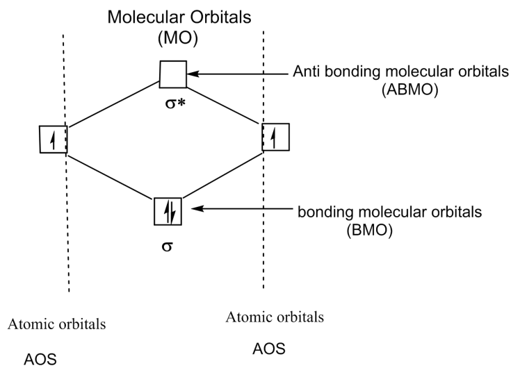
Fig. 4.28 picture of the molecular orbital diagram.
