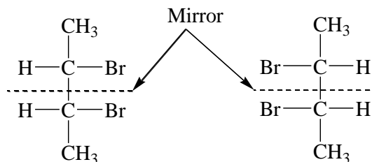
2,3-Dibromobutane
