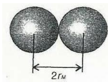
Fig. 3.3 Metallic radius
