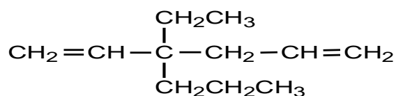
3-ethyl-3-propylhexa-1,5-diene
