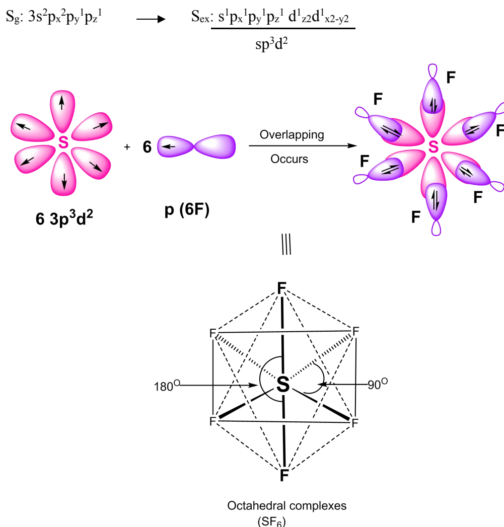
Fig 4.16 Formation of six \sigma covalent bonds by the overlapping of sp^3d^2 hybrid orbitals of S central atom with p -orbitals of six F atoms
