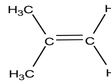
2-Methylpropene
