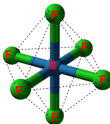
3-D modal of Octahedral complex
