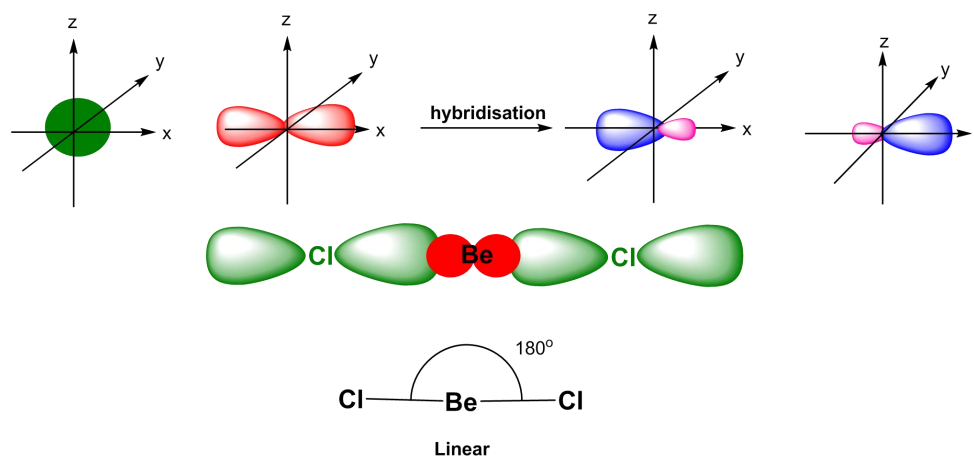
Fig 4.7 Formation of two collinear sp hybrid orbitals from the mixing of one s and one p atomic orbitals ( sp hybridisation)
