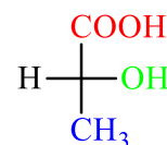
Fischer projection
