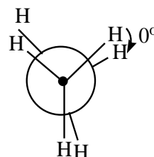
Eclipsed conformation
