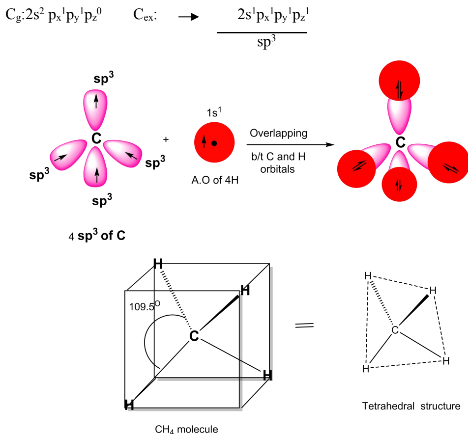
Fig 4.12 formation of four \sigma covalent bonds by the overlapping of sp^3 hybrid orbitals of C-atom and 1s orbitals of four H-atoms
