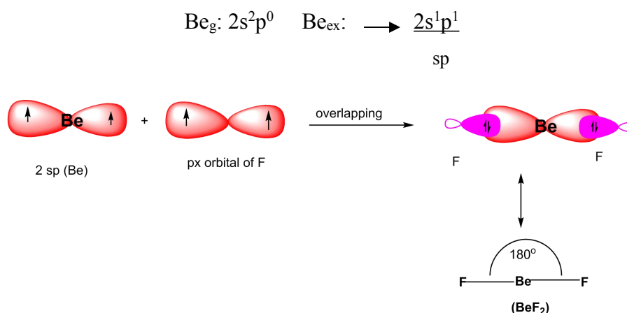
Fig 4.8 formation of two \sigma covalent bonds by the overlapping of sp -hybrid orbitals of \text{Be} and 2p -orbitals of \text{F} -atoms
