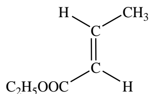
trans -ethylbutenoate
