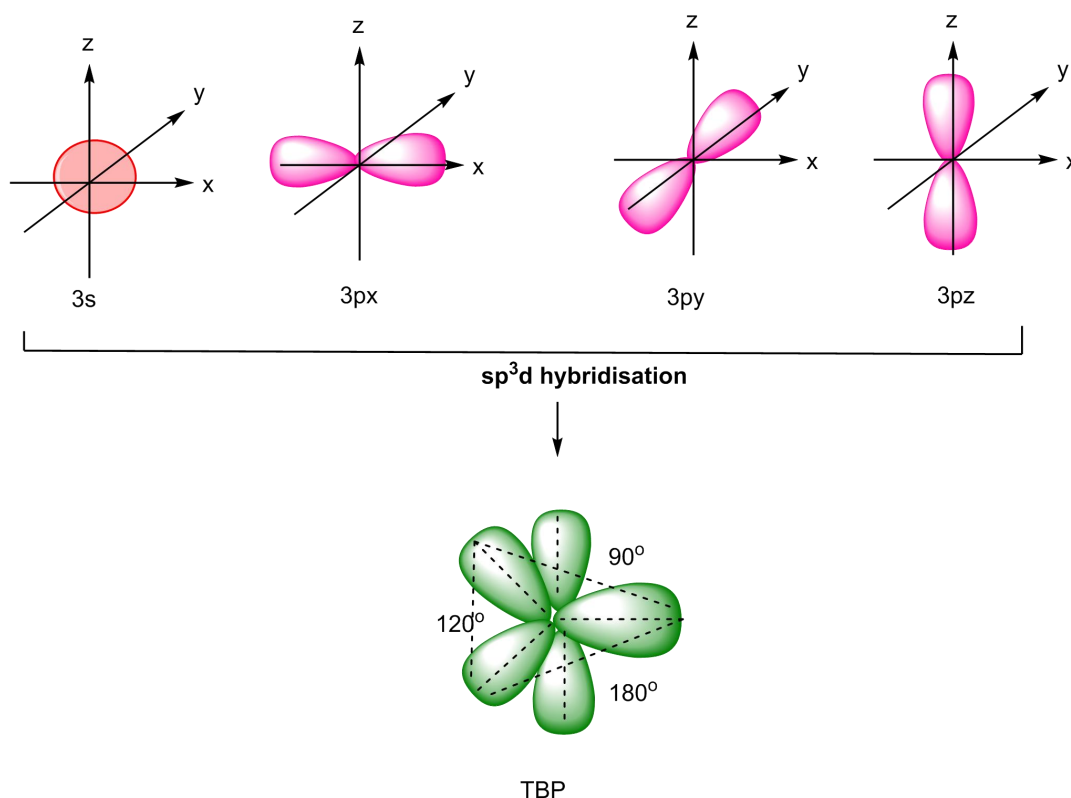
Fig 4.13 formation of five trigonal bipyramidal sp^3d hybrid orbitals from the mixing of one s , three p and one d ( d_{z^2} ) atomic orbitals ( sp^3d hybridisation).
