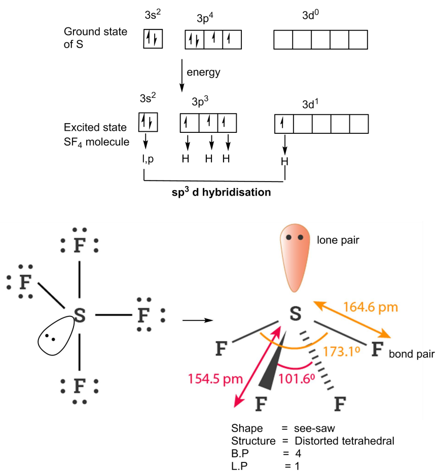
Fig 4.22 Formation of five hybrid orbitals of S_{ex} atom and their overlapping with p-orbitals of four F-atom to give SF_4 molecule
