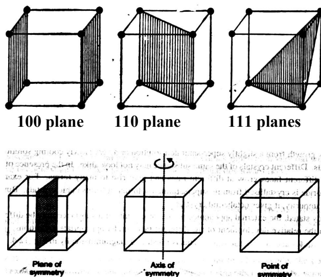
Fig 12.8 three cubic unit cells
