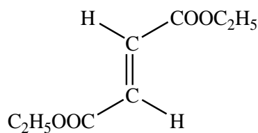
diethyl fumarate
