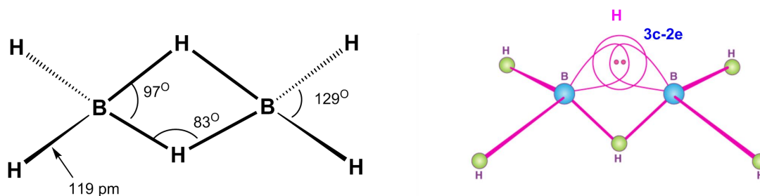
4.35 Structure of the diborane
