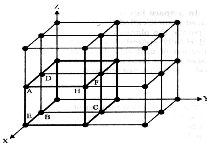
Fig 12.3 Space lattice
