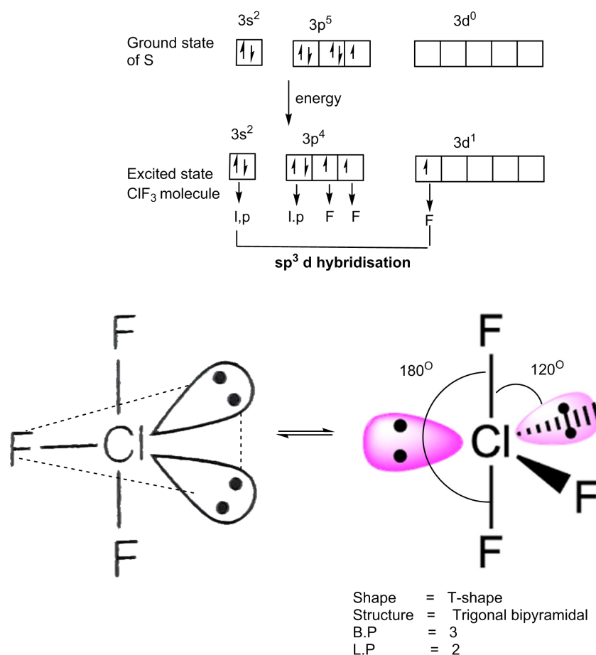
Fig 4.23 Formation of five hybrid orbitals of \text{Cl}_1^{\text{st}_{\text{ex}}} atom and their overlapping with p-orbitals of three F-atoms to give \text{ClF}_3 molecule
