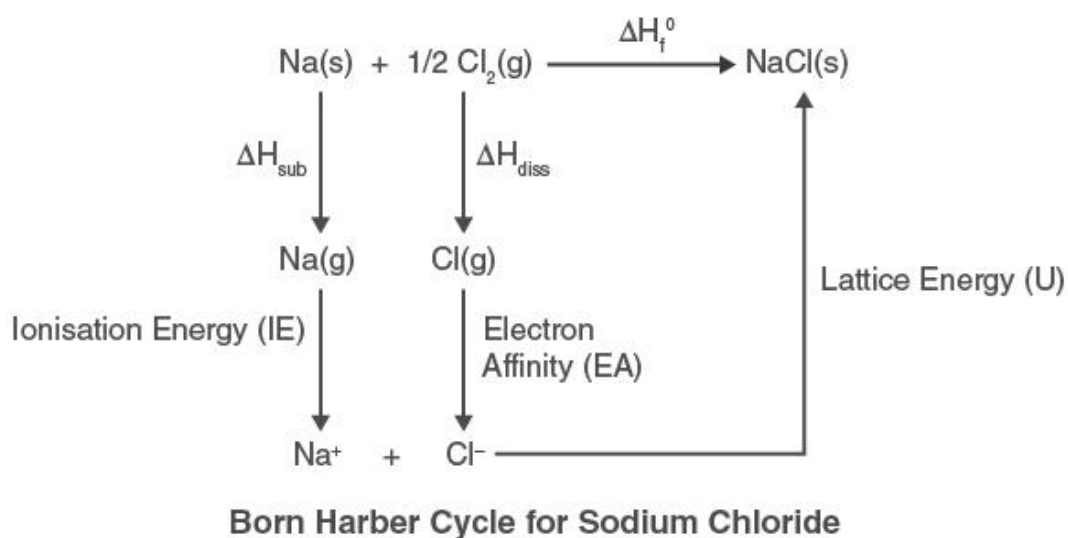
Fig 12.16 Born-Haber cycle
