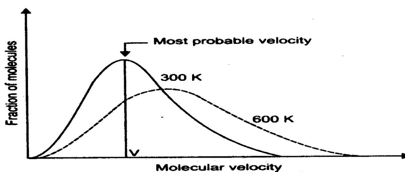
Fig 11.1 Distribution of molecular velocities at two temperatures.
