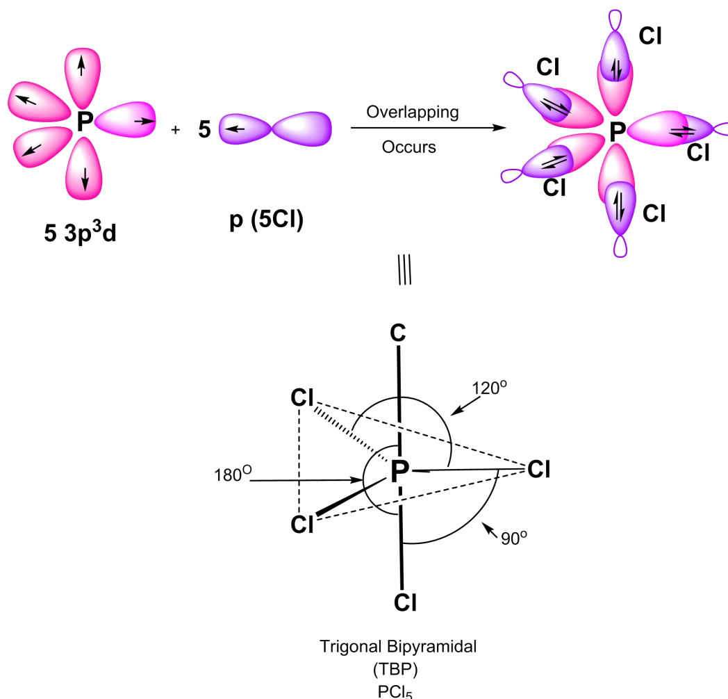
Fig 4.14 Formation of five \sigma covalent bonds by the overlapping of sp^3d hybrid orbitals of P central atom and p-orbitals of five Cl-atoms
