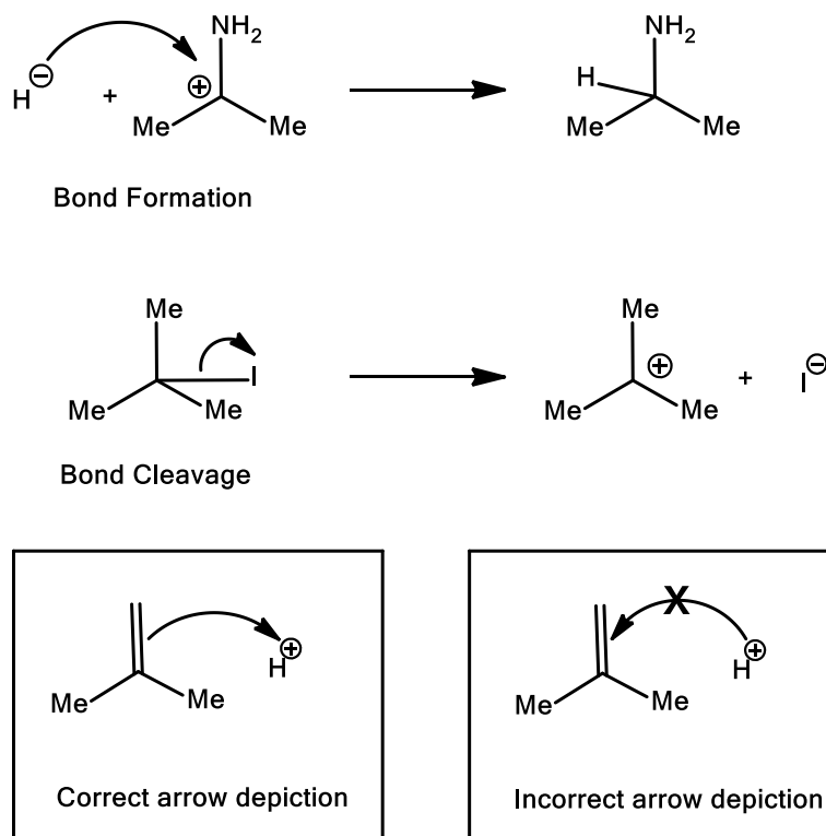
Figure 5.4 Correct depiction of curved arrow for formation and breaking of covalent bond. Inset images show correct and incorrect way to depict electron movement with curved arrows.
