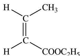
cis -ethylbutenoate
