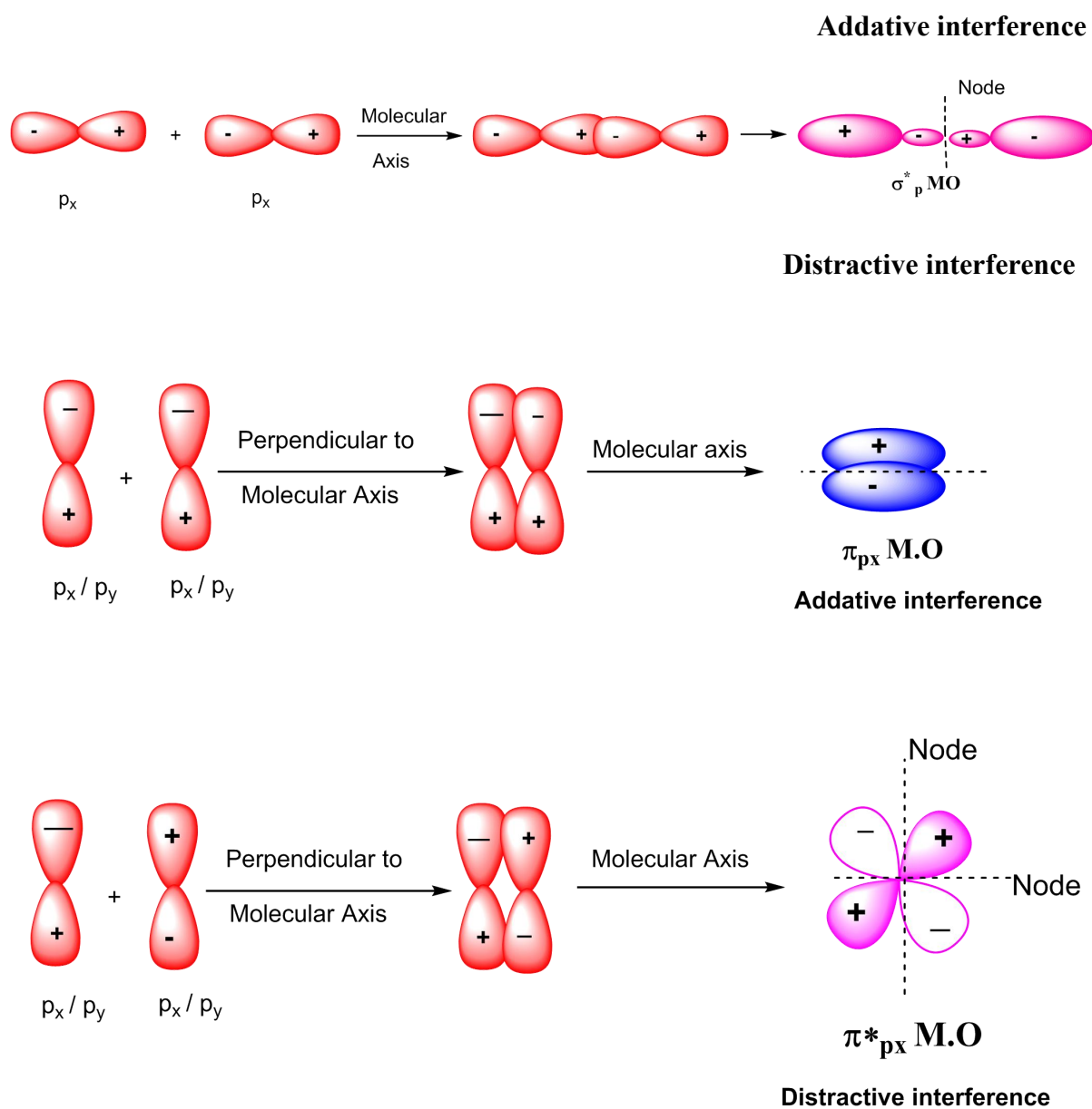
Fig. 4.29 picture of the various combination of atomic orbital.
