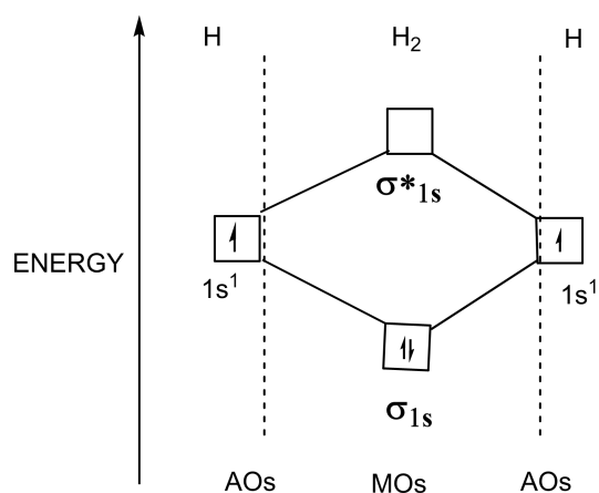
Fig 4.30 Energy level diagram of H 2
