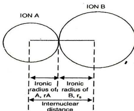
Fig. 3.4 The ionic radius
