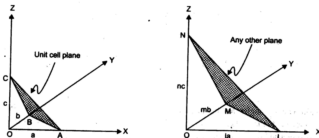
Fig 12.5 A unit cell plane intercepts the axes to give intercepts a, b and c
