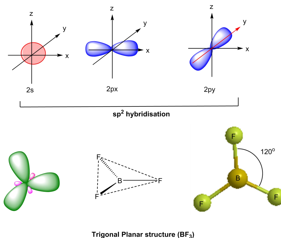
Fig 4.9 Formation of three trigonal planar sp^2 hybrid orbitals from the mixing of one s and two p atomic orbitals ( sp^2 hybridisation).
