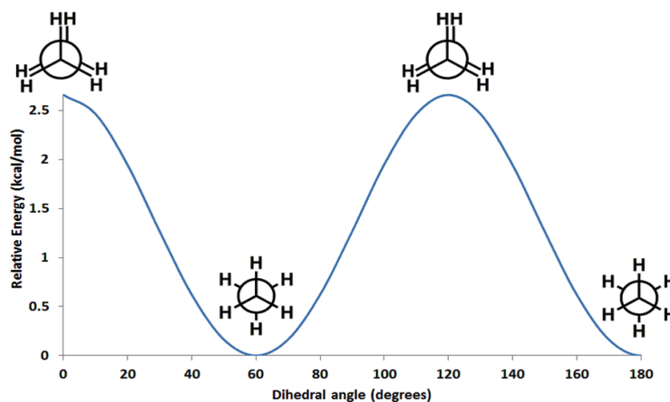
Figure 7.1: Energy profile diagram of conformational isomer of ethane
